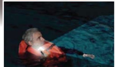
The SOLAS PML has a battery operated, water or manually activated beacon in addition to the chemical light. Electronics will shut off 30 minutes after being removed from the water
